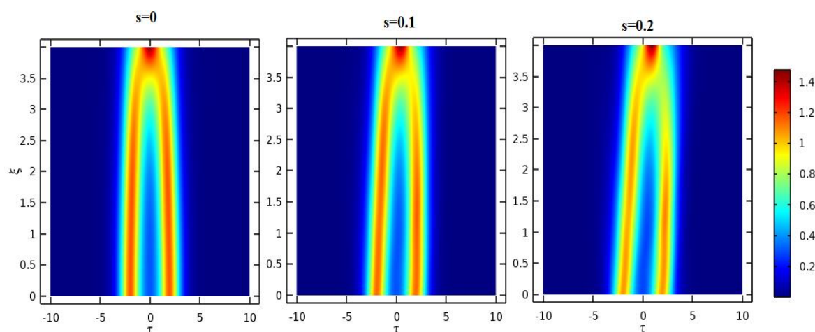
Figure 18: Soliton Interaction For N=1 At T_R = \delta_3 = 0, q = 2, r = 1, \phi = 0 For Many Values Of s
