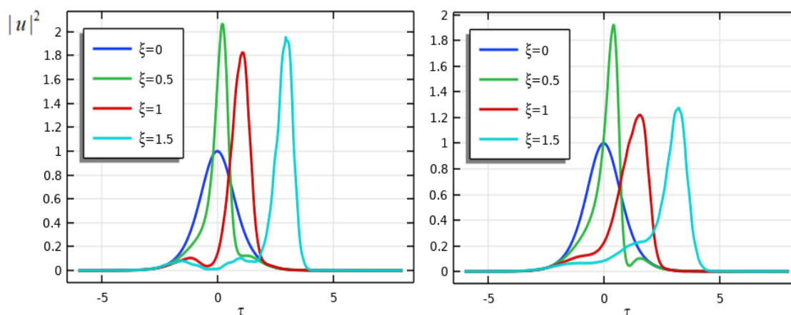
Figure 12: Pulse Evolution For N=2 Soliton At s = 0, \delta_3 = 0.002 And T_R = 0.1, 0.2 , Respectively
