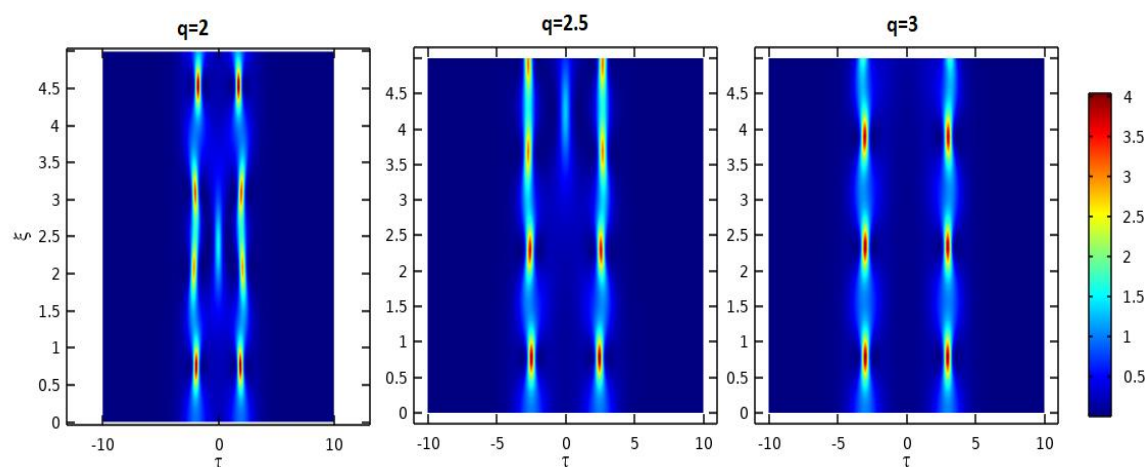
Figure 14: Soliton Interaction For N=2 At \phi = s = T_R = \delta_3 = 0, r = 1 For Many Values Of q
