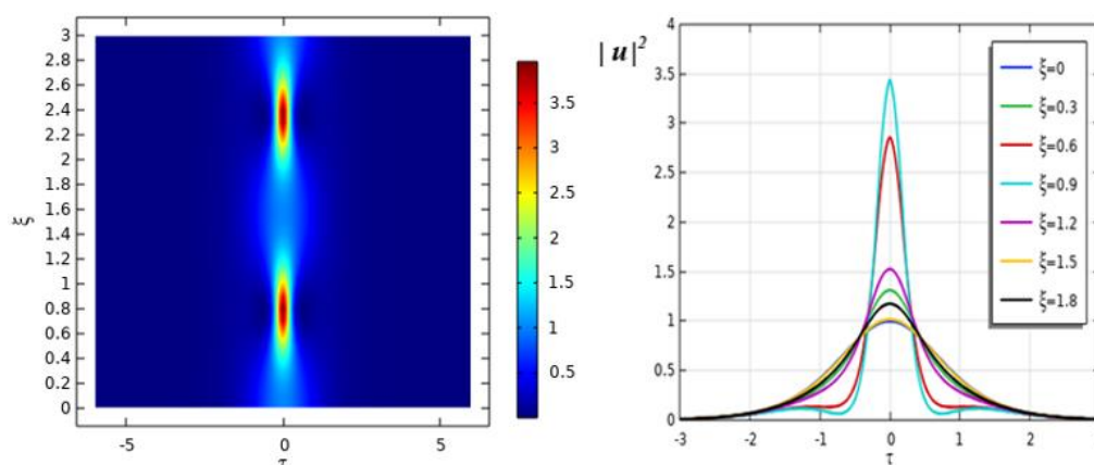
Figure 2: pulse evolution for N=2 soliton at zero chirp
