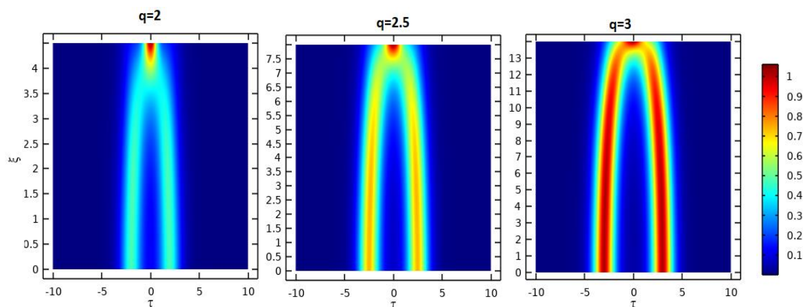
Figure 13: Soliton Interaction for N=1 at \phi = s = T_R = \delta_3 = 0, r = 1 For Many Values Of q
