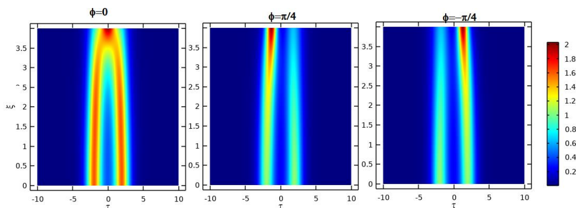
Figure 17: Soliton Interaction For N=1 At s = T_R = \delta_3 = 0, q = 2, r = 1 For Many Values Of \phi
