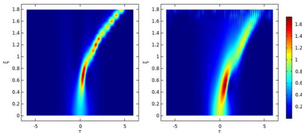
Figure 6: Pulse Evolution for N=2 Soliton At s = 0, \delta_3 = 0 and T_R = 0.1, 0.3 , Respectively
