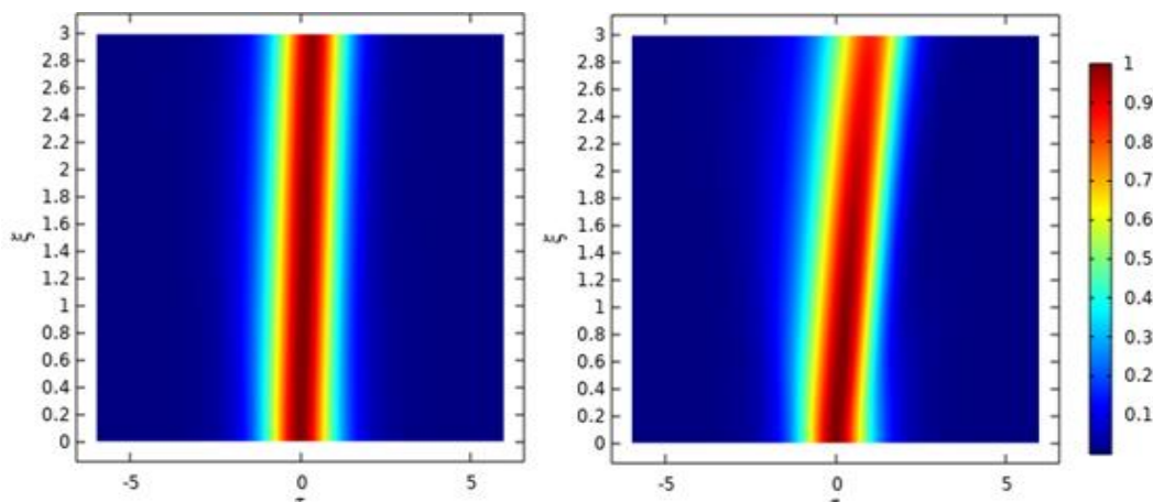
Figure 5: Pulse Evolution for N=1 Soliton At s = 0, \delta_3 = 0 and T_R = 0.1, 0.3 , Respectively
