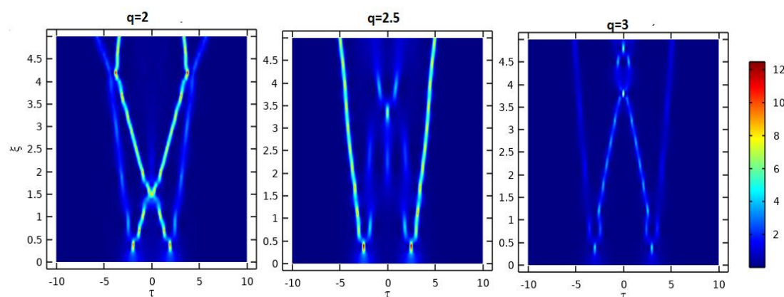
Figure 15: Soliton Interaction For N=3 At \phi = s = T_R = \delta_3 = 0, r = 1 For Many Values Of q
