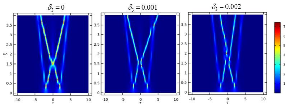
Figure 20: soliton interaction for N=3 at s = T_R = 0, q = 2, r = 1, \phi = 0 for many values of \delta_3
