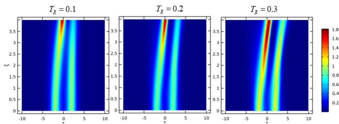
Figure 19: Soliton Interaction For N=1 At s = \delta_3 = 0, q = 2, r = 1, \phi = 0 For Many Values Of T_R
