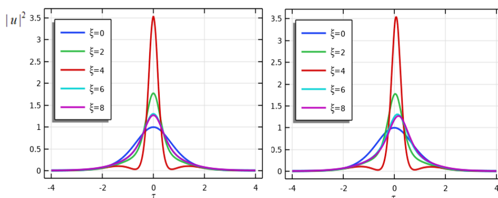
Figure 10: Pulse Evolution for N=2 Soliton At T_R = 0, s = 0 and \delta_3 = 0, 0.002 , Respectively
