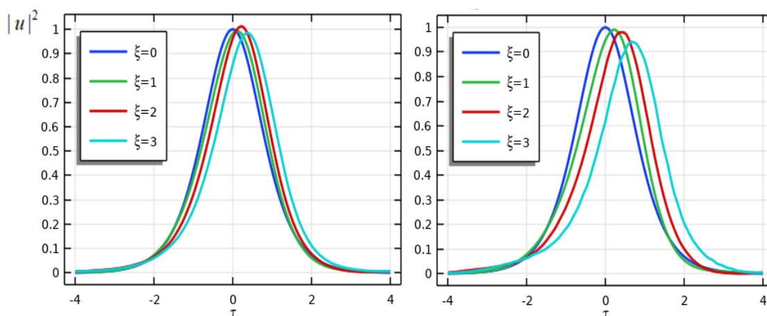
Figure 11: Pulse Evolution For N=1 Soliton At s = 0, \delta_3 = 0.002 And T_R = 0.1, 0.2 , Respectively
